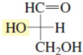
(S)-(-)-glyceraldehyde
