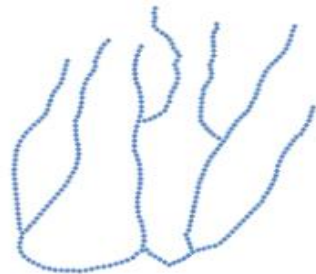
amylopectin
