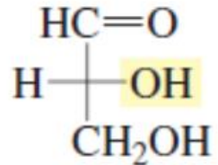
(R)-(+)-glyceraldehyde
